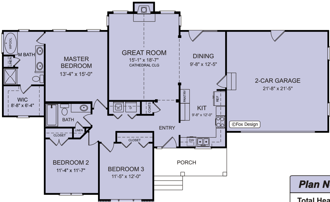
Floor Plan
