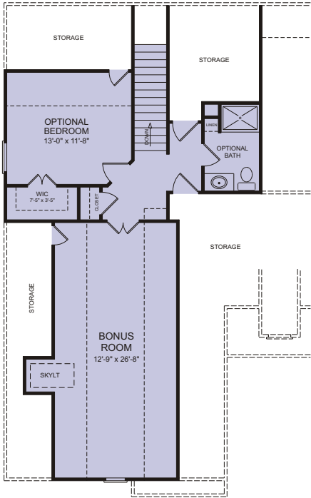
Bonus Room Plan
