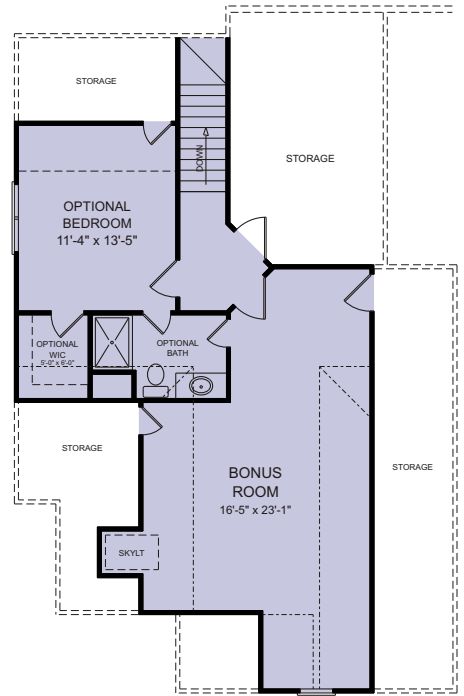
Bonus Room Plan
